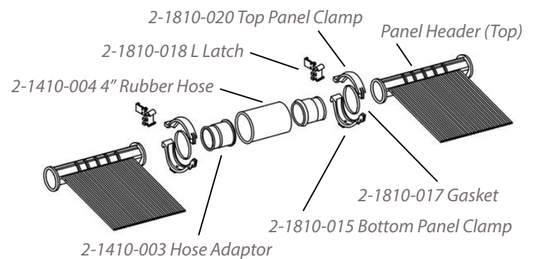
7B. Hose Adaptor Connection Method
