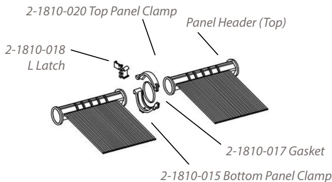
7A. Panel Clamp Connection Method
